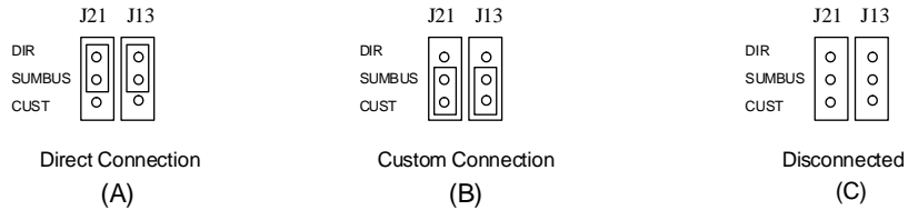
Figure 10. SUMBUS Jumper Settings
